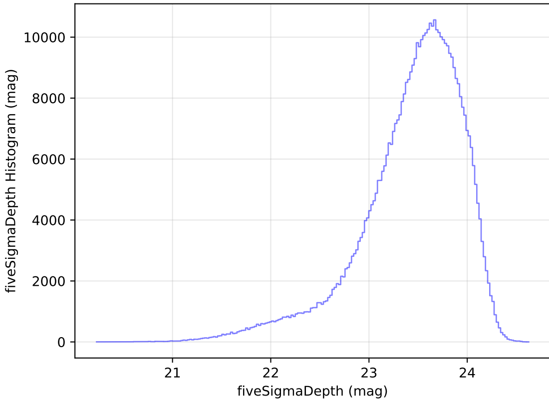
weather_cloudso30v3.4_10yrs WFD i band: fiveSigmaDepth Histogram
