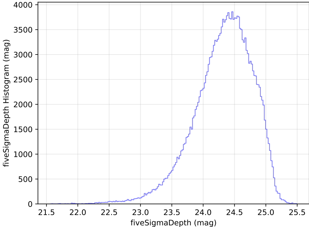
weather_cloudso30v3.4_10yrs WFD g band: fiveSigmaDepth Histogram
