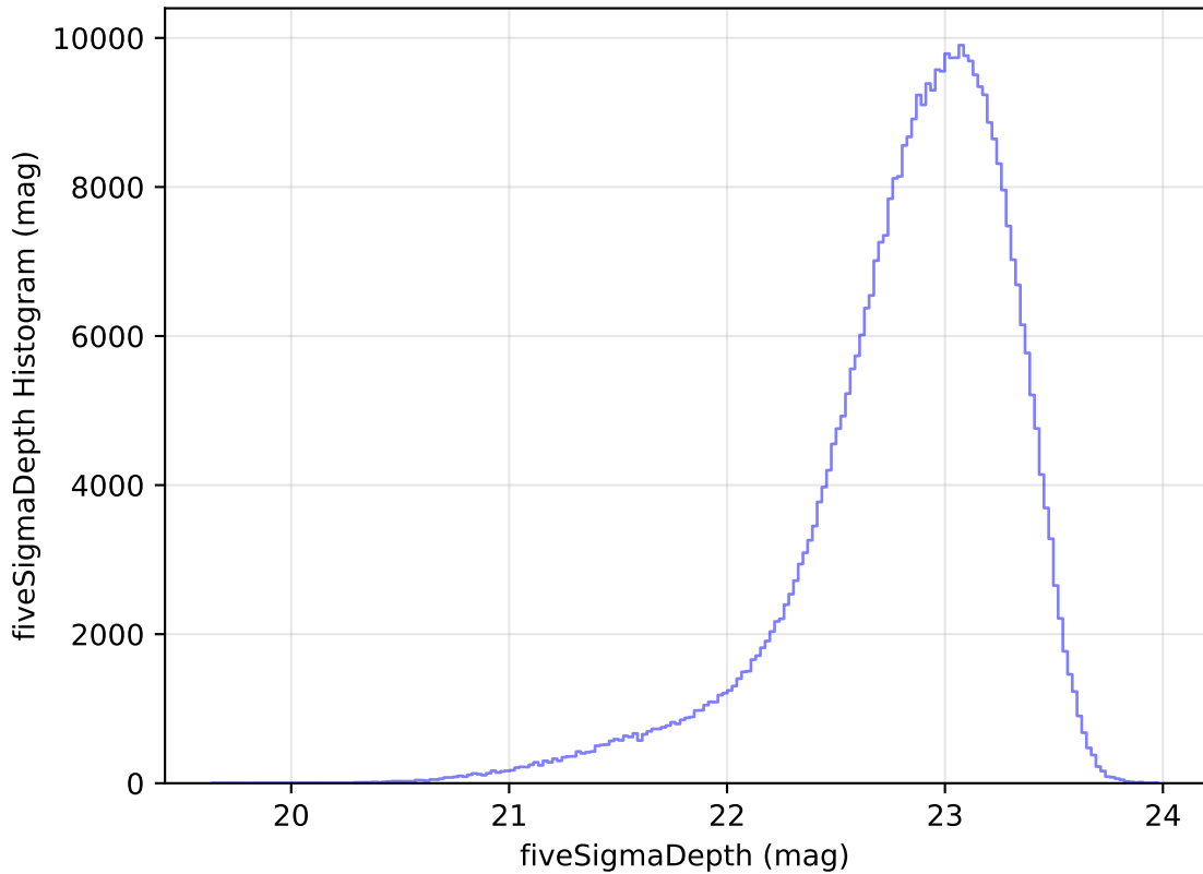
weather_cloudso30v3.4_10yrs All sky z band: fiveSigmaDepth Histogram
