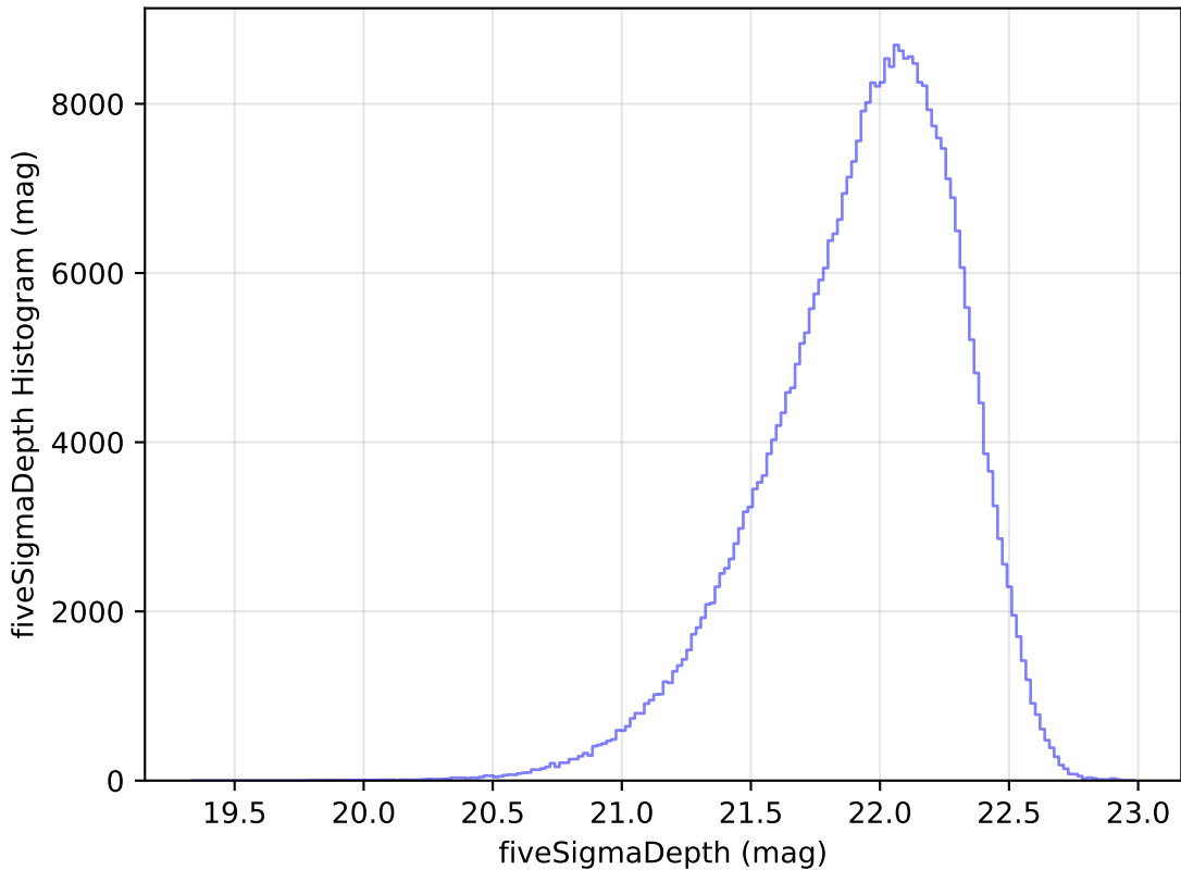
weather_cloudso30v3.4_10yrs All sky y band: fiveSigmaDepth Histogram
