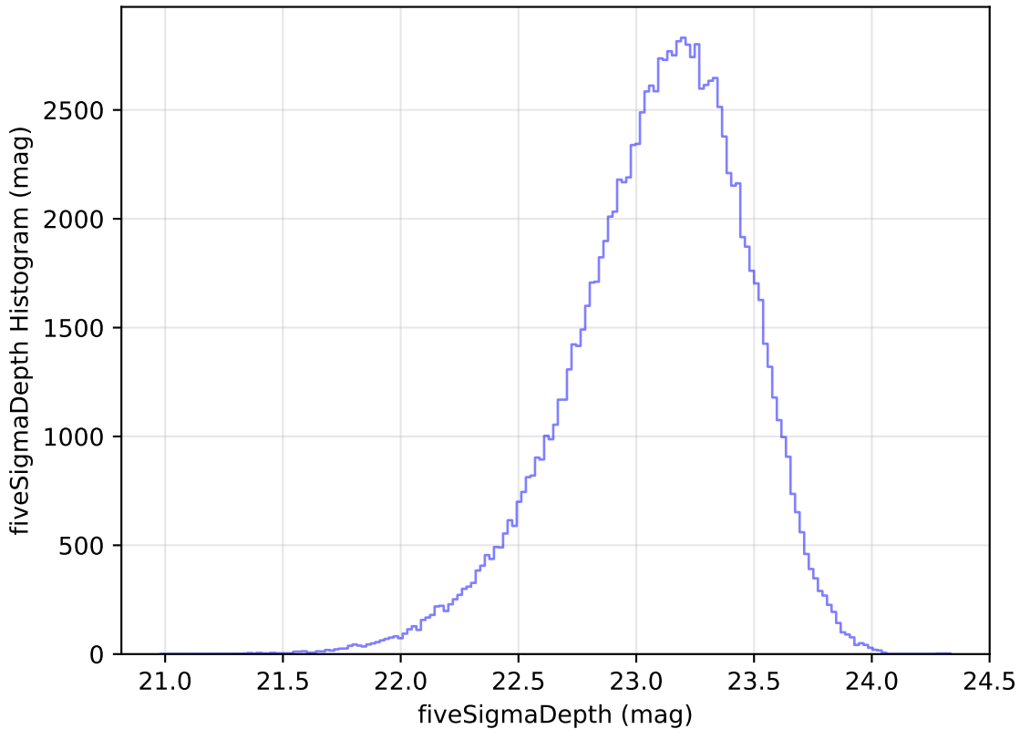
weather_cloudso30v3.4_10yrs All sky u band: fiveSigmaDepth Histogram
