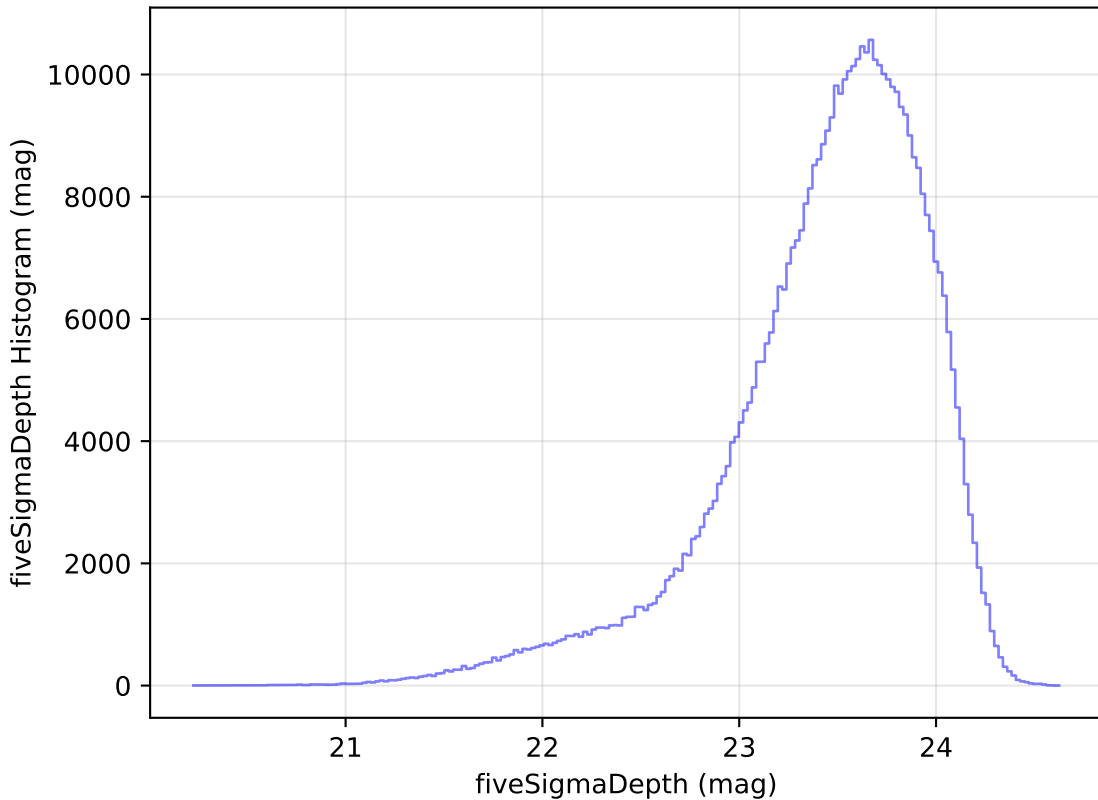
weather_cloudso30v3.4_10yrs All sky i band: fiveSigmaDepth Histogram
