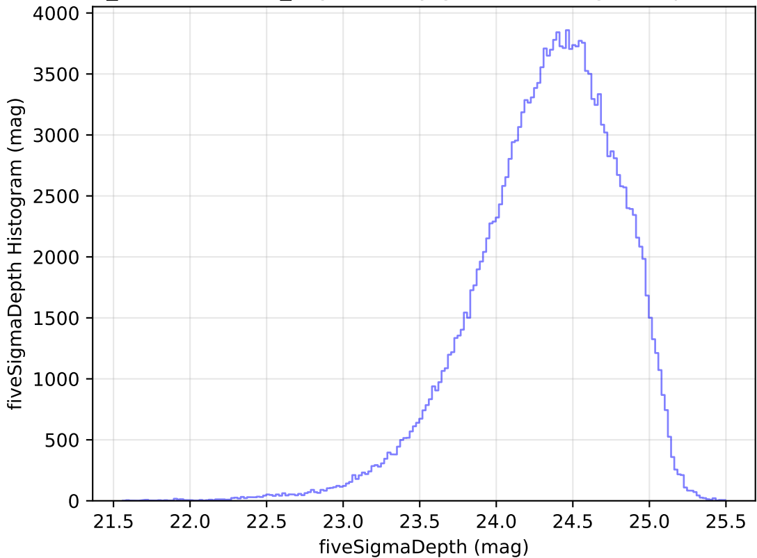
weather_cloudso30v3.4_10yrs All sky g band: fiveSigmaDepth Histogram
