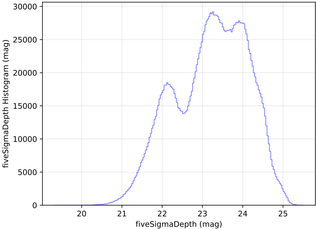
weather_cloudso30v3.4_10yrs All sky all bands: fiveSigmaDepth Histogram
