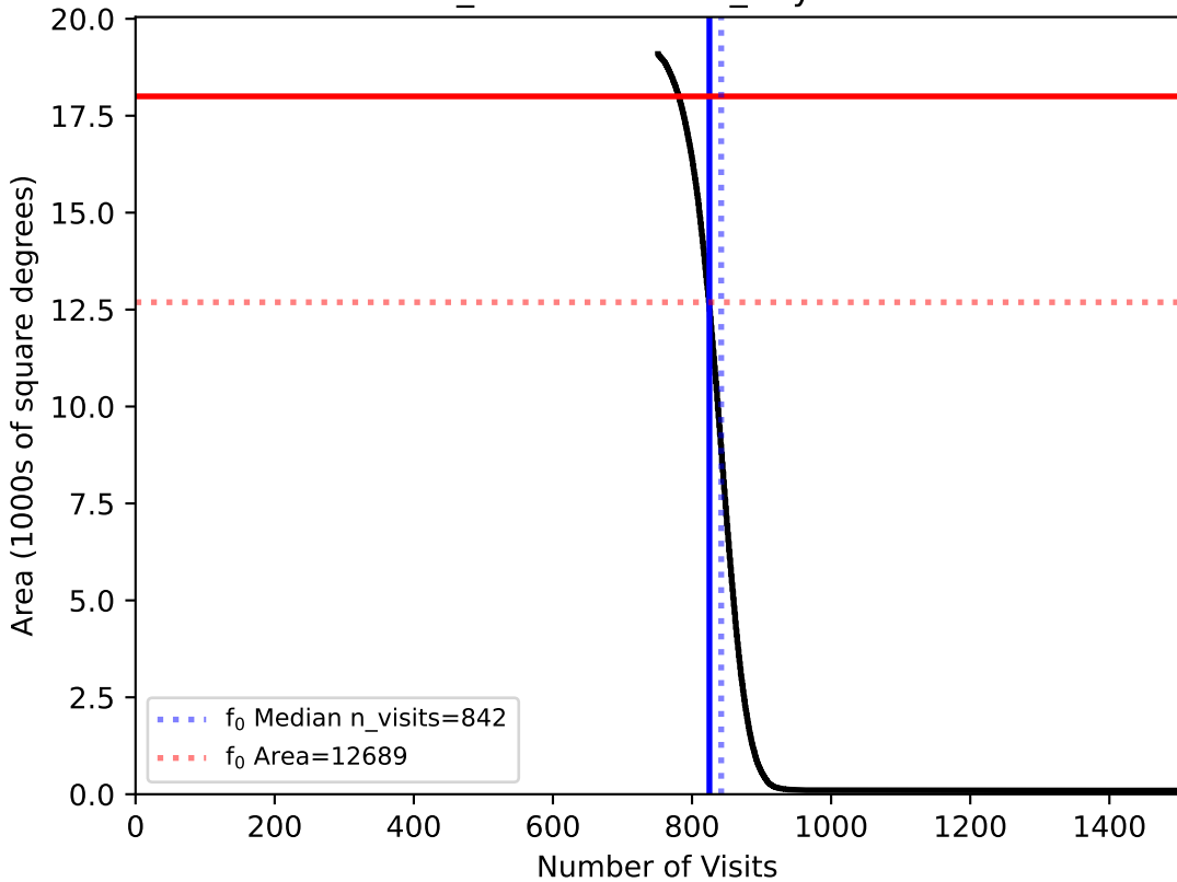
weather_cloudso30v3.4_10yrs WFD: f0
