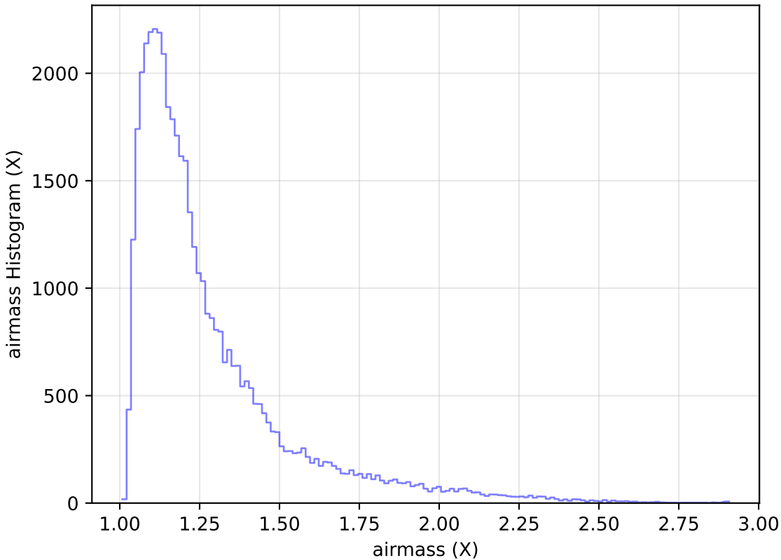
weather_cloudso30v3.4_10yrs Yr 1 y band: airmass Histogram
