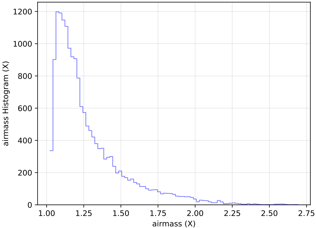
weather_cloudso30v3.4_10yrs Yr 1 u band: airmass Histogram
