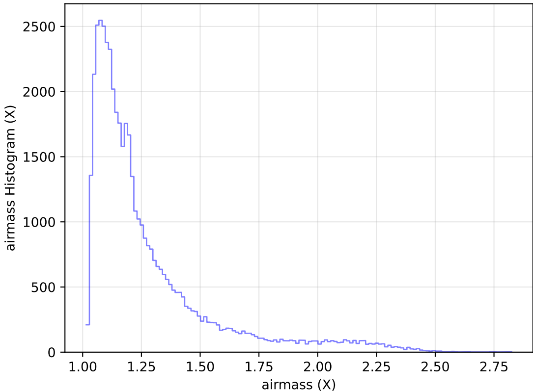
weather_cloudso30v3.4_10yrs Yr 1 r band: airmass Histogram
