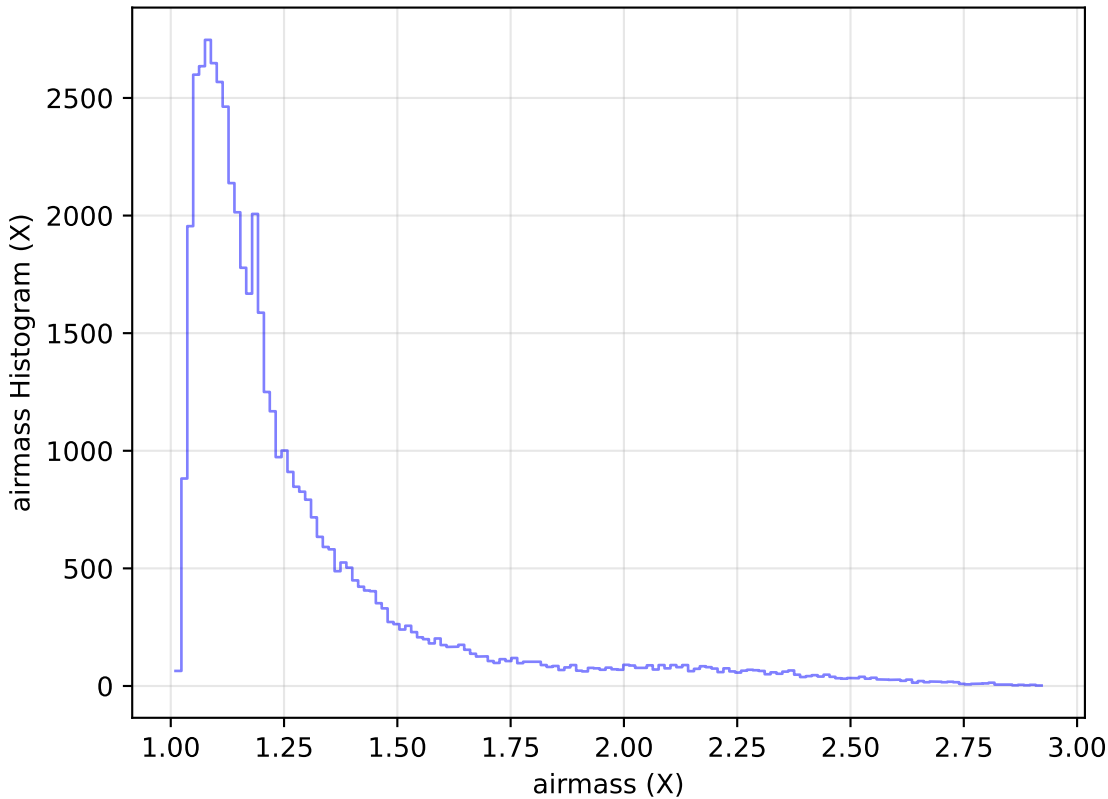
weather_cloudso30v3.4_10yrs Yr 1 i band: airmass Histogram
