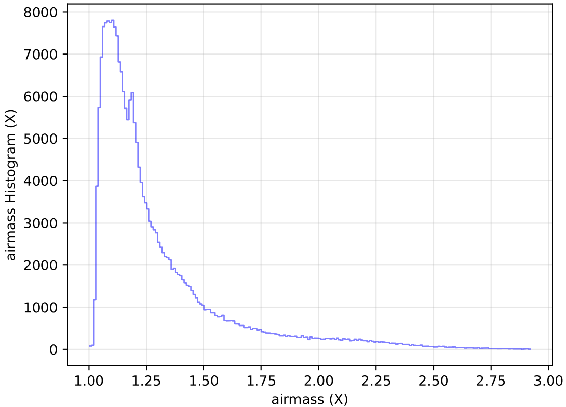
weather_cloudso30v3.4_10yrs Yr 1 all bands: airmass Histogram
