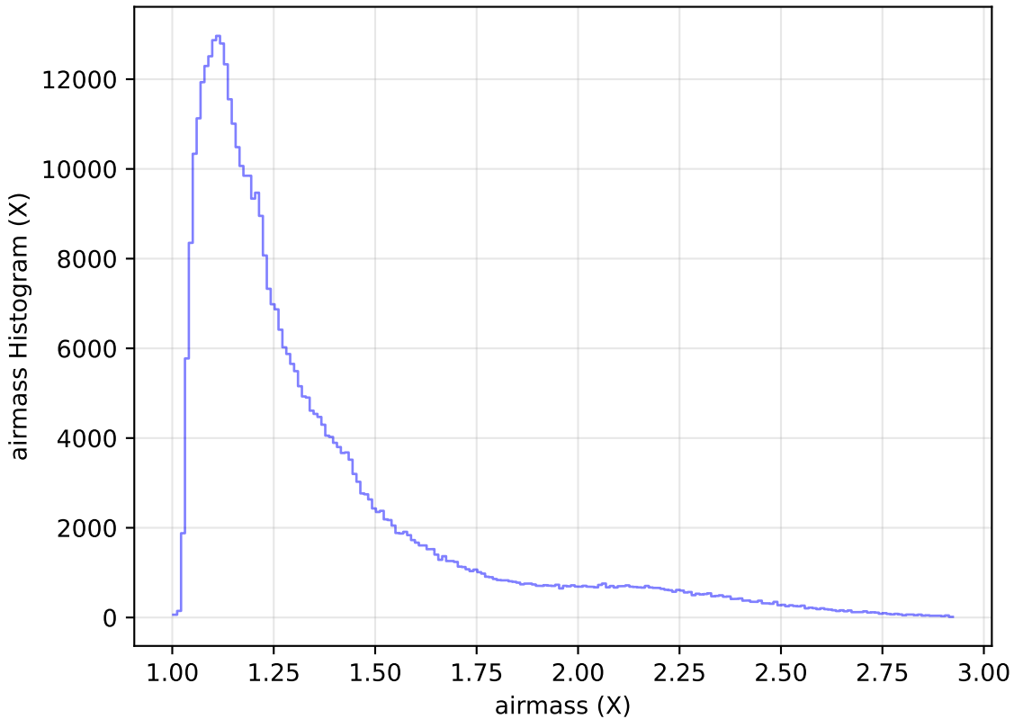
weather_cloudso30v3.4_10yrs WFD z band: airmass Histogram
