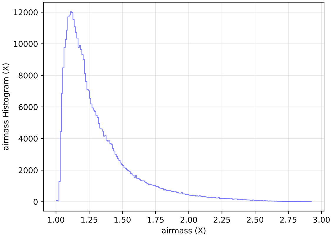
weather_cloudso30v3.4_10yrs WFD y band: airmass Histogram
