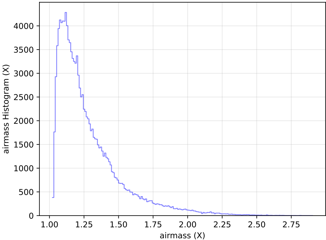
weather_cloudso30v3.4_10yrs WFD u band: airmass Histogram
