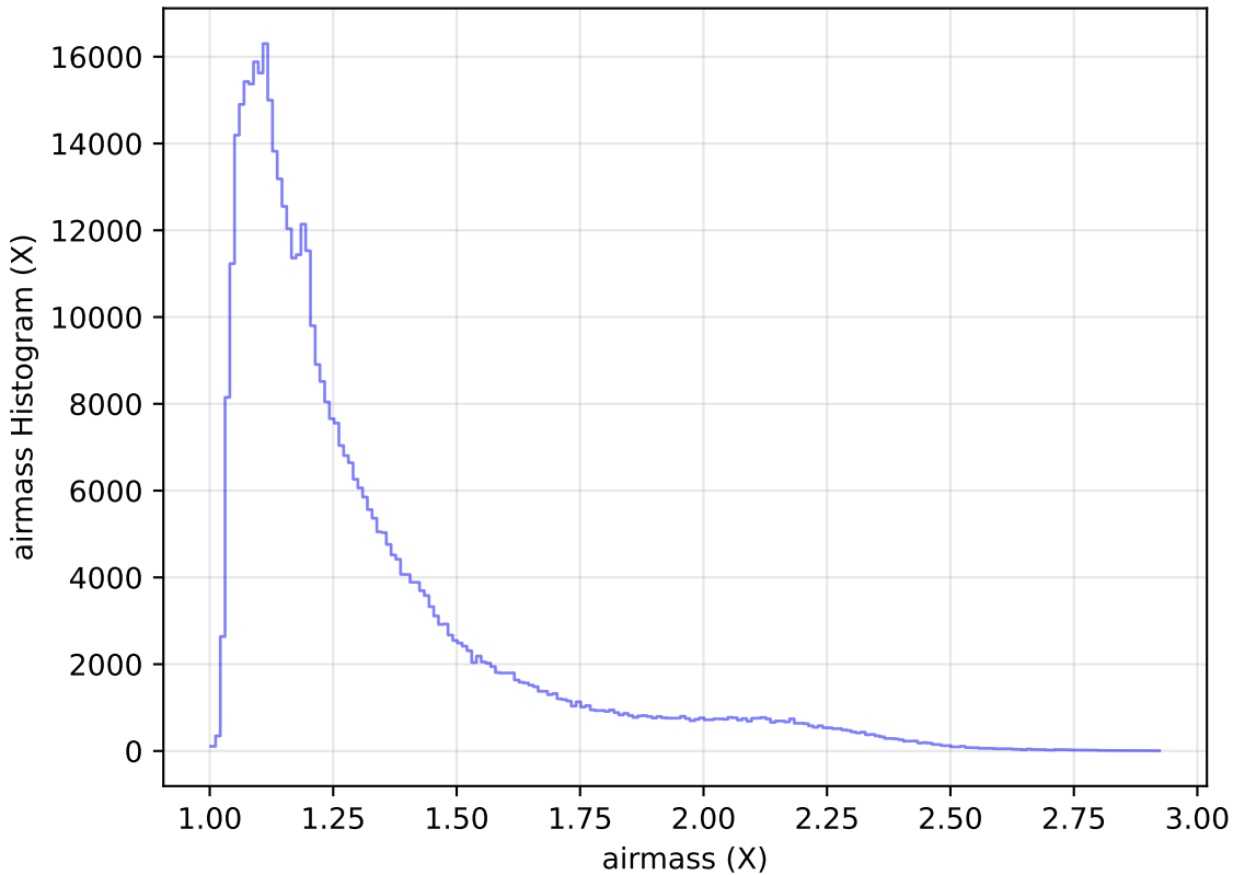
weather_cloudso30v3.4_10yrs WFD r band: airmass Histogram
