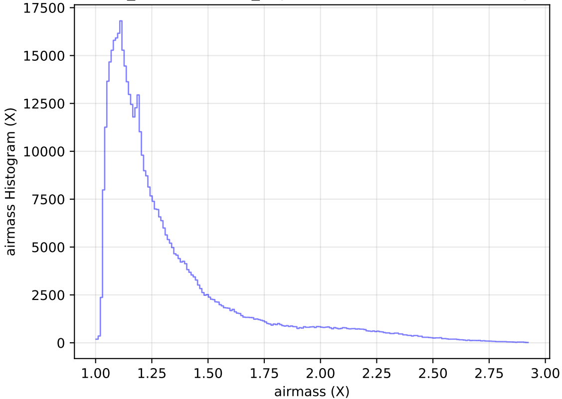
weather_cloudso30v3.4_10yrs WFD i band: airmass Histogram
