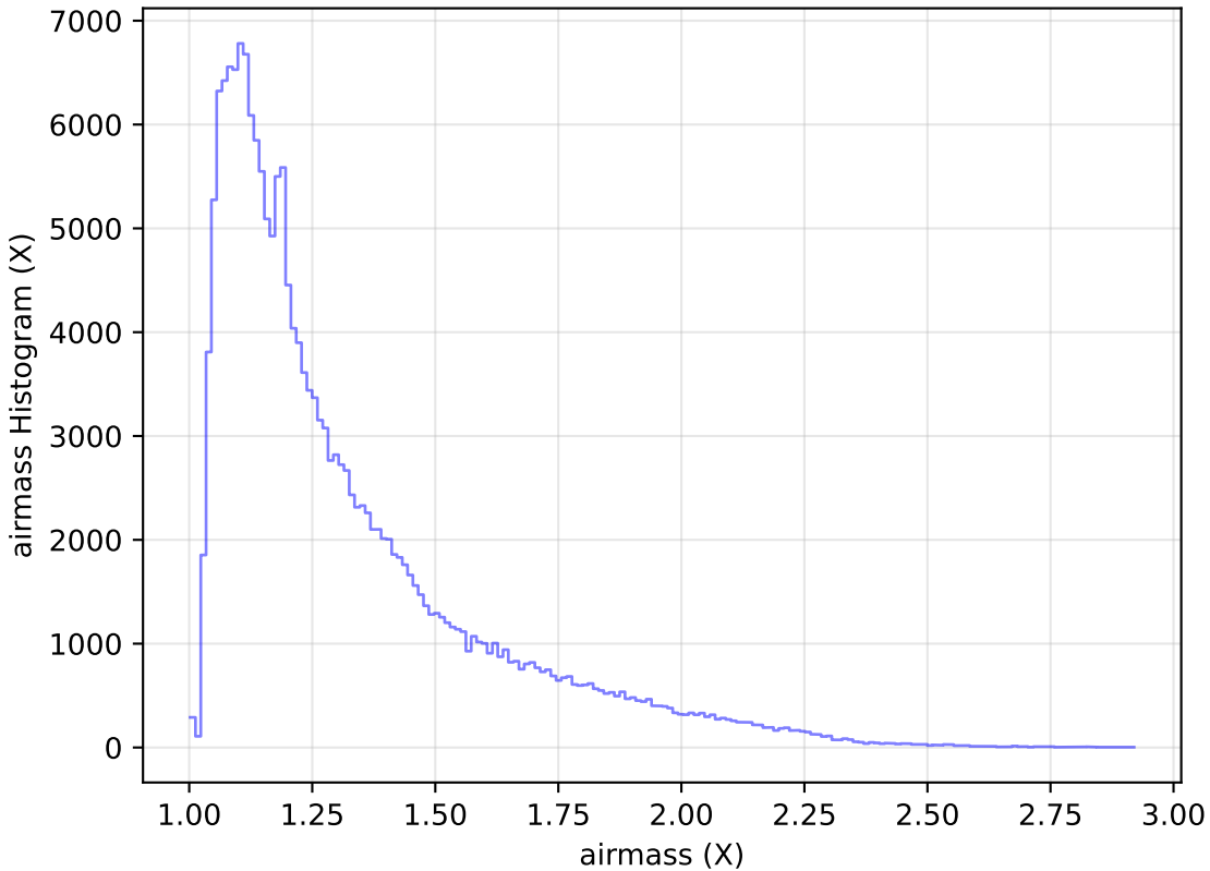
weather_cloudso30v3.4_10yrs WFD g band: airmass Histogram
