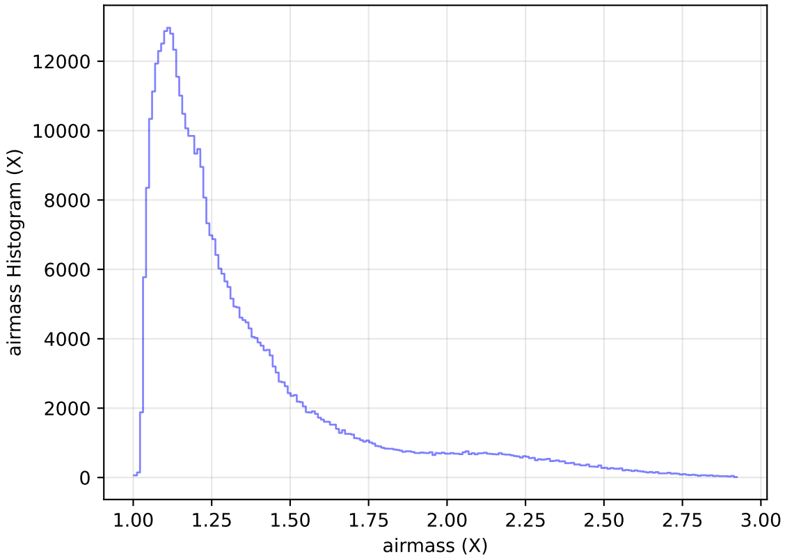
weather_cloudso30v3.4_10yrs All sky z band: airmass Histogram
