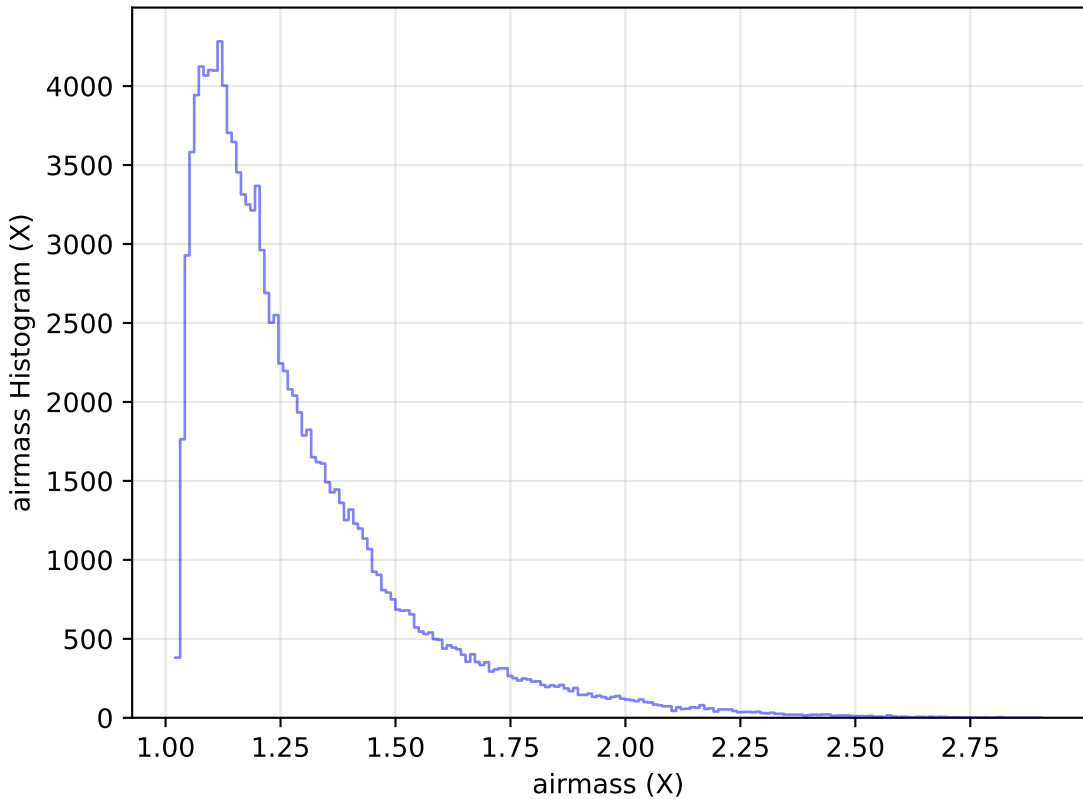
weather_cloudso30v3.4_10yrs All sky u band: airmass Histogram
