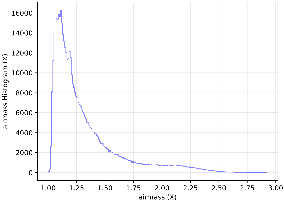
weather_cloudso30v3.4_10yrs All sky r band: airmass Histogram
