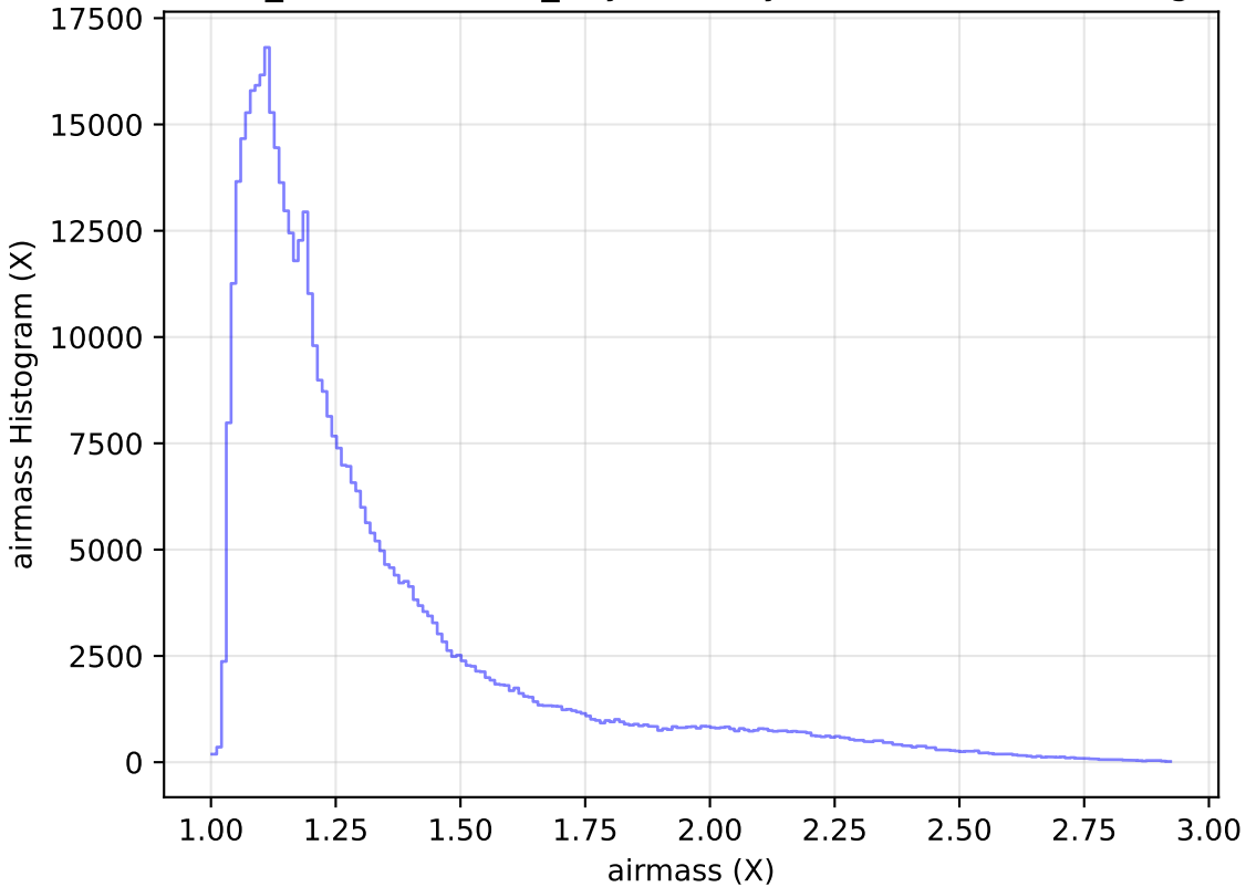
weather_cloudso30v3.4_10yrs All sky i band: airmass Histogram
