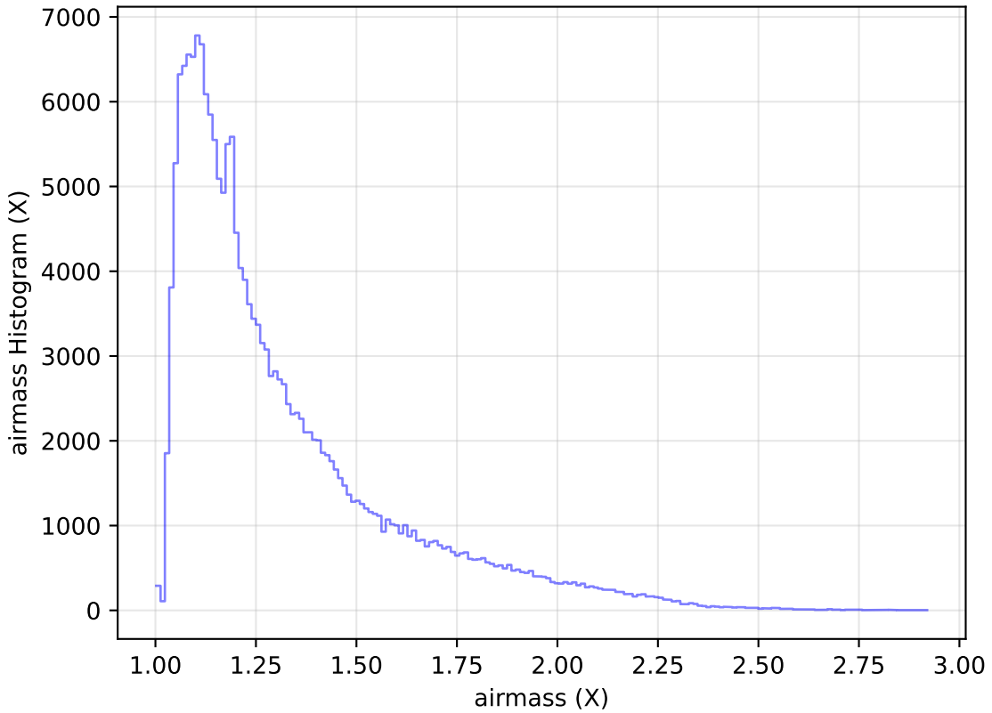
weather_cloudso30v3.4_10yrs All sky g band: airmass Histogram
