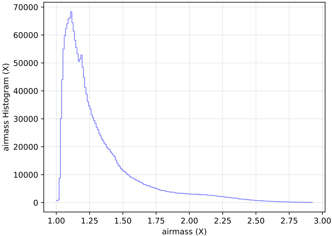
weather_cloudso30v3.4_10yrs All sky all bands: airmass Histogram
