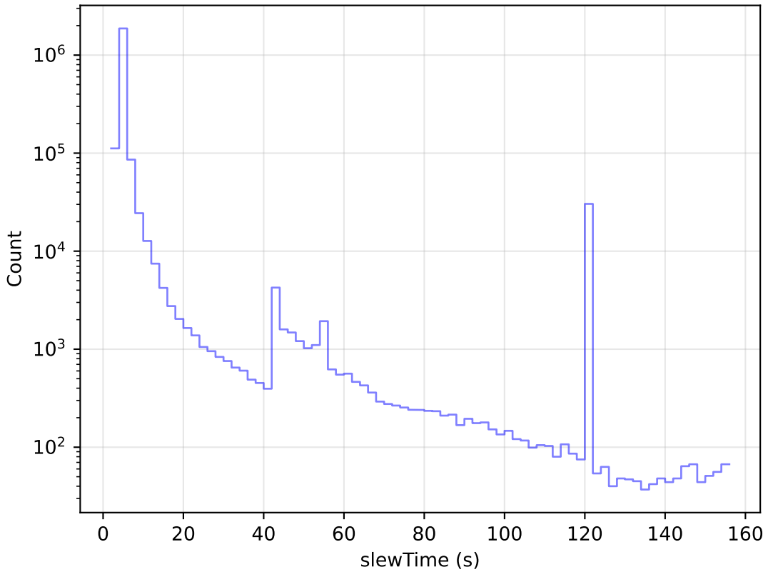
weather_cloudso30v3.4_10yrs All visits: Slew Time Histogram
