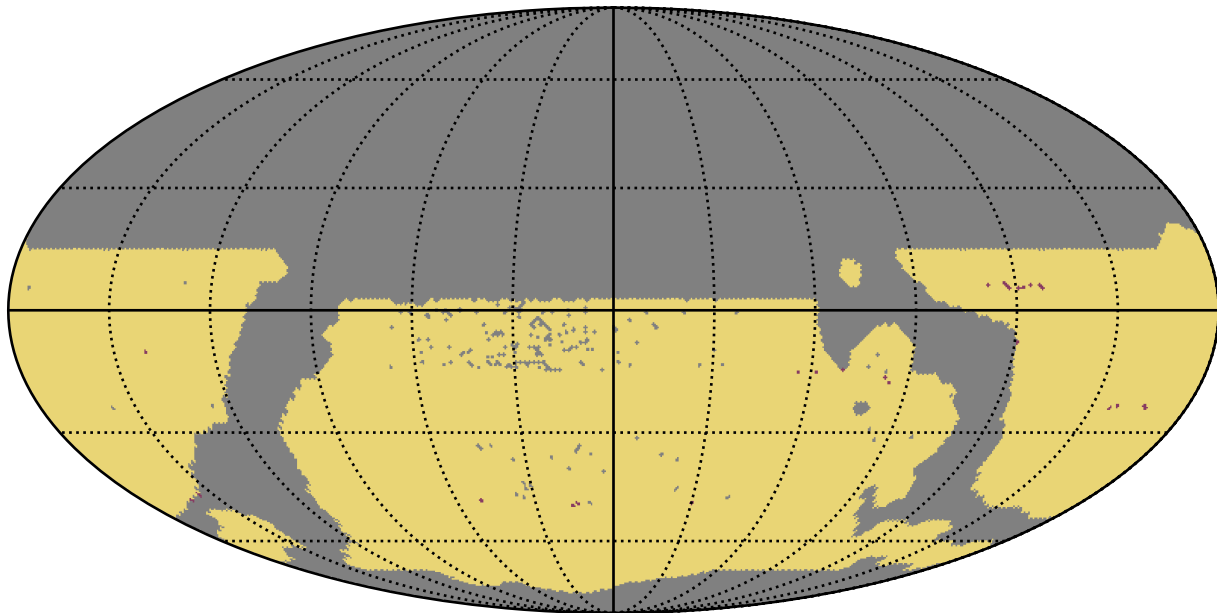
weather_cloudso30v3.4_10yrs WFD: RapidRevisits
