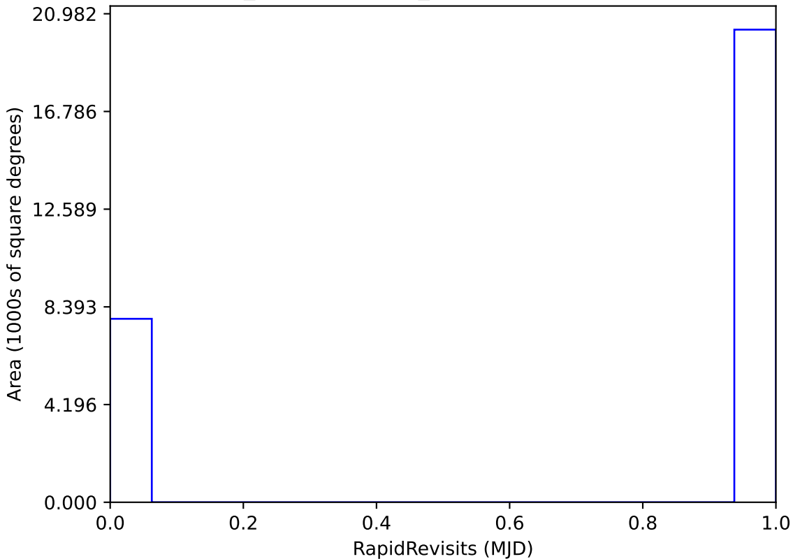
weather_cloudso30v3.4_10yrs All sky: RapidRevisits
