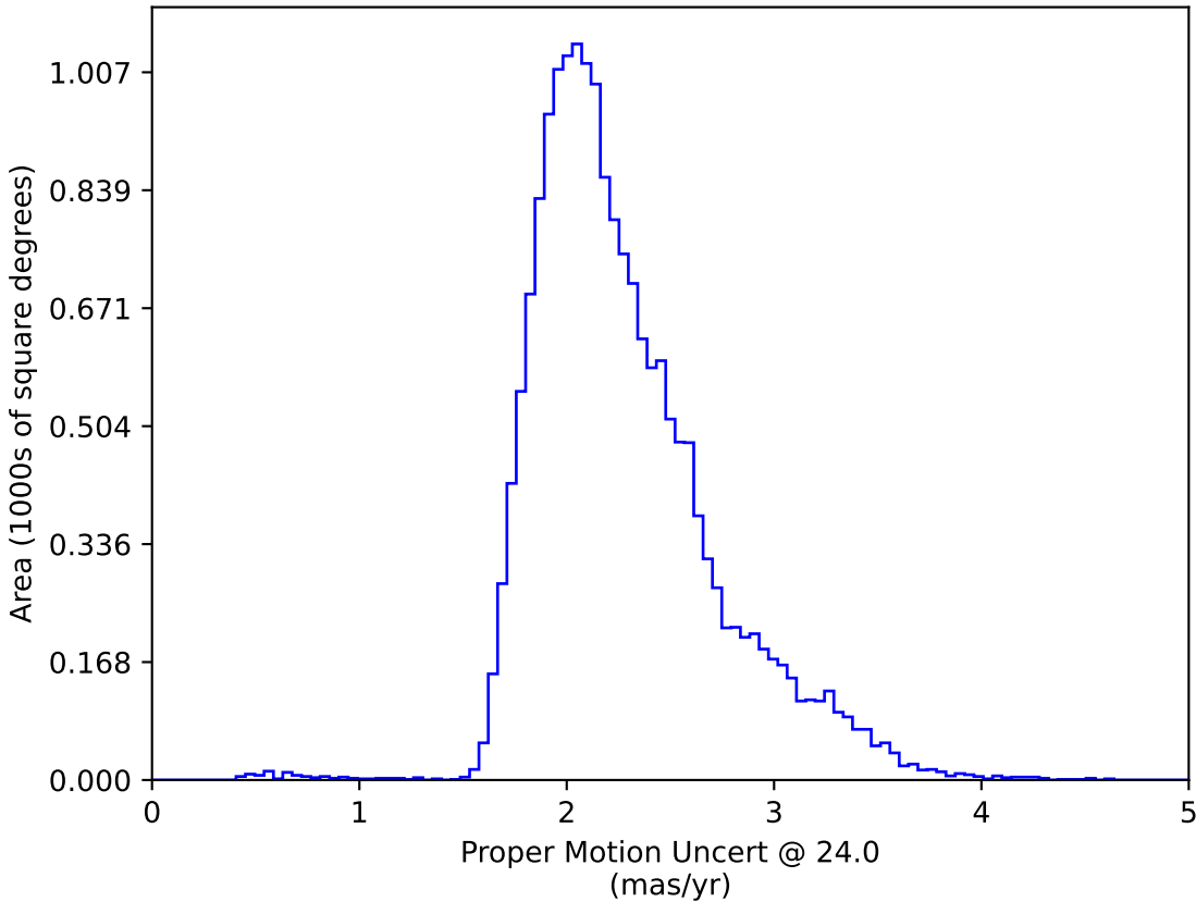
weather_cloudso30v3.4_10yrs WFD: Proper Motion Uncert @ 24.0
