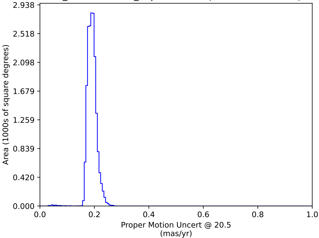
weather_cloudso30v3.4_10yrs WFD: Proper Motion Uncert @ 20.5
