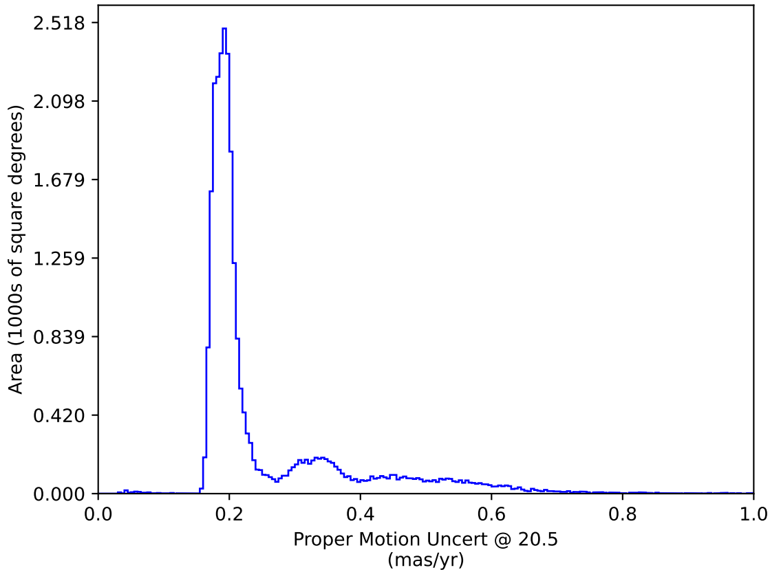
weather_cloudso30v3.4_10yrs All sky: Proper Motion Uncert @ 20.5
