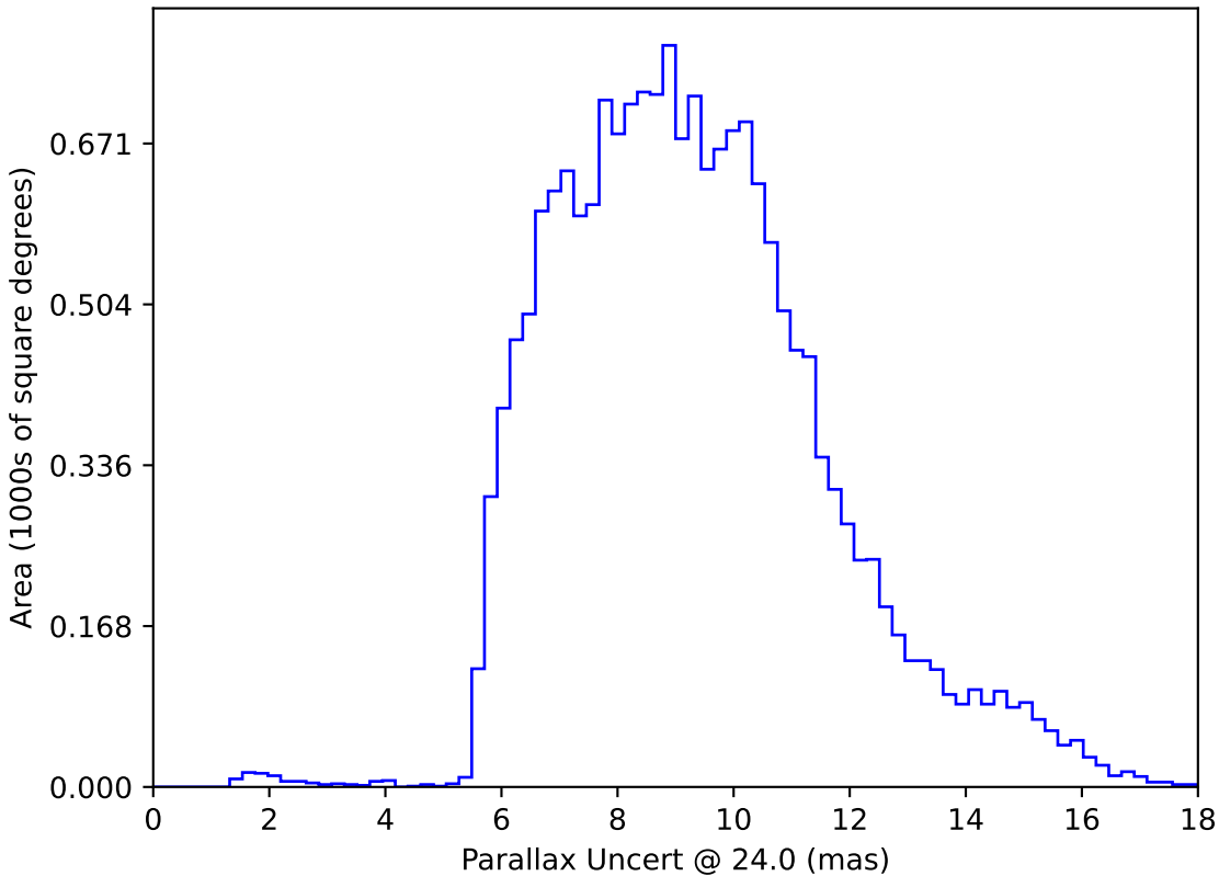
weather_cloudso30v3.4_10yrs WFD: Parallax Uncert @ 24.0
