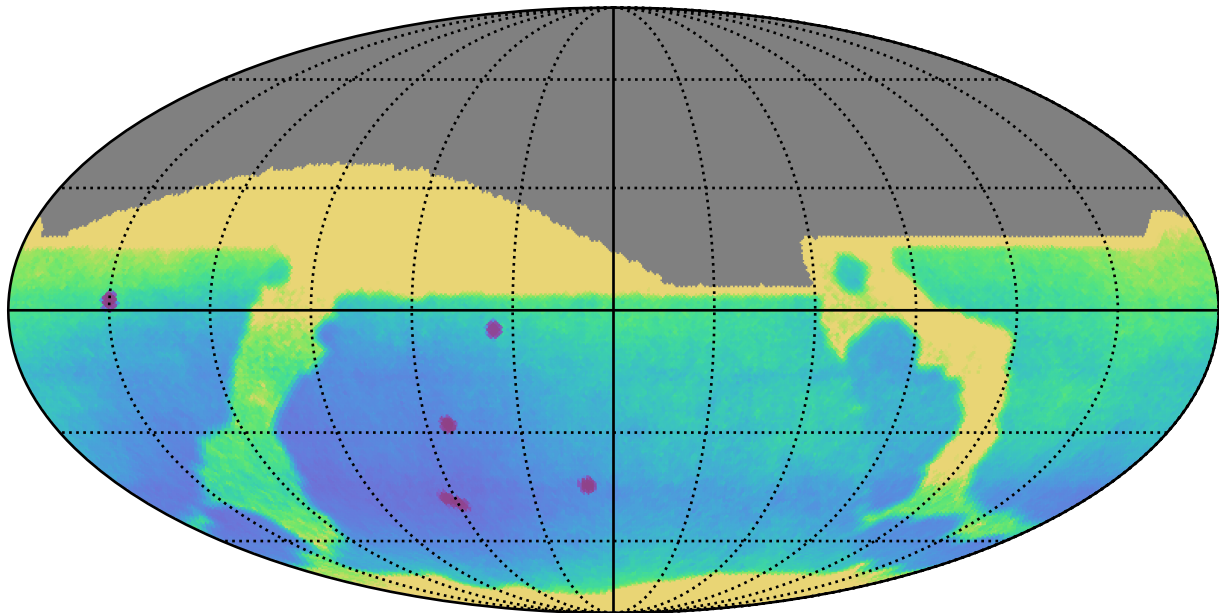
weather_cloudso30v3.4_10yrs All sky: Parallax Uncert @ 24.0
