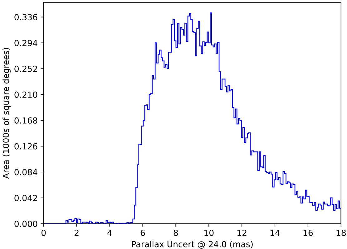
weather_cloudso30v3.4_10yrs All sky: Parallax Uncert @ 24.0
