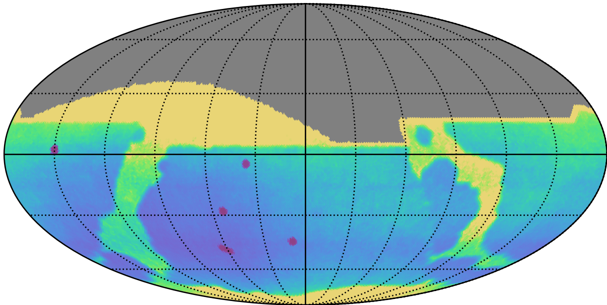
weather_cloudso30v3.4_10yrs All sky: Parallax Uncert @ 22.4
