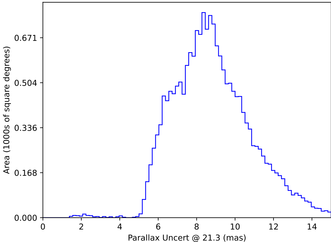
weather_cloudso30v3.4_10yrs WFD y band only: Parallax Uncert @ 21.3
