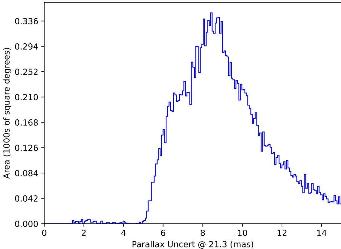
weather_cloudso30v3.4_10yrs All sky y band only: Parallax Uncert @ 21.3
