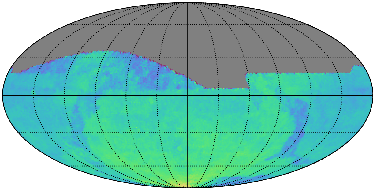
weather_cloudso30v3.4_10yrs All sky: Parallax Coverage @ 24.0
