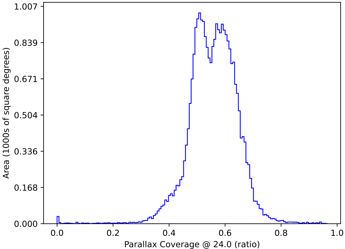
weather_cloudso30v3.4_10yrs All sky: Parallax Coverage @ 24.0
