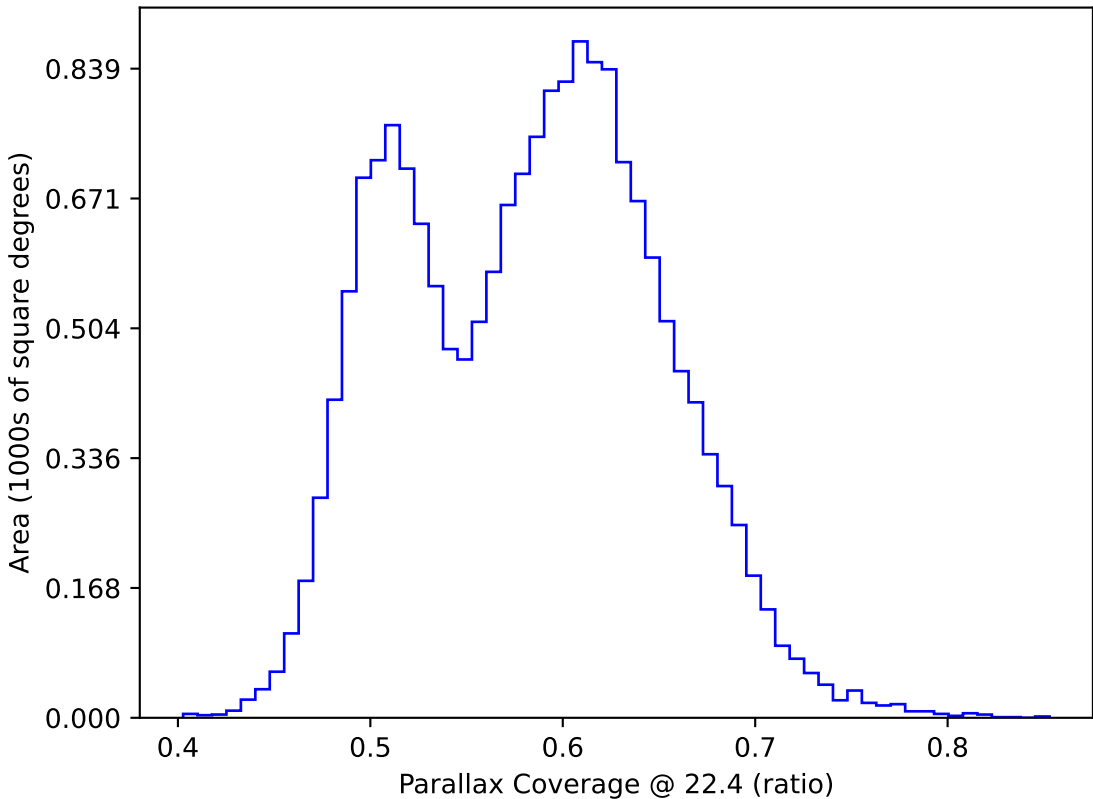
weather_cloudso30v3.4_10yrs WFD: Parallax Coverage @ 22.4
