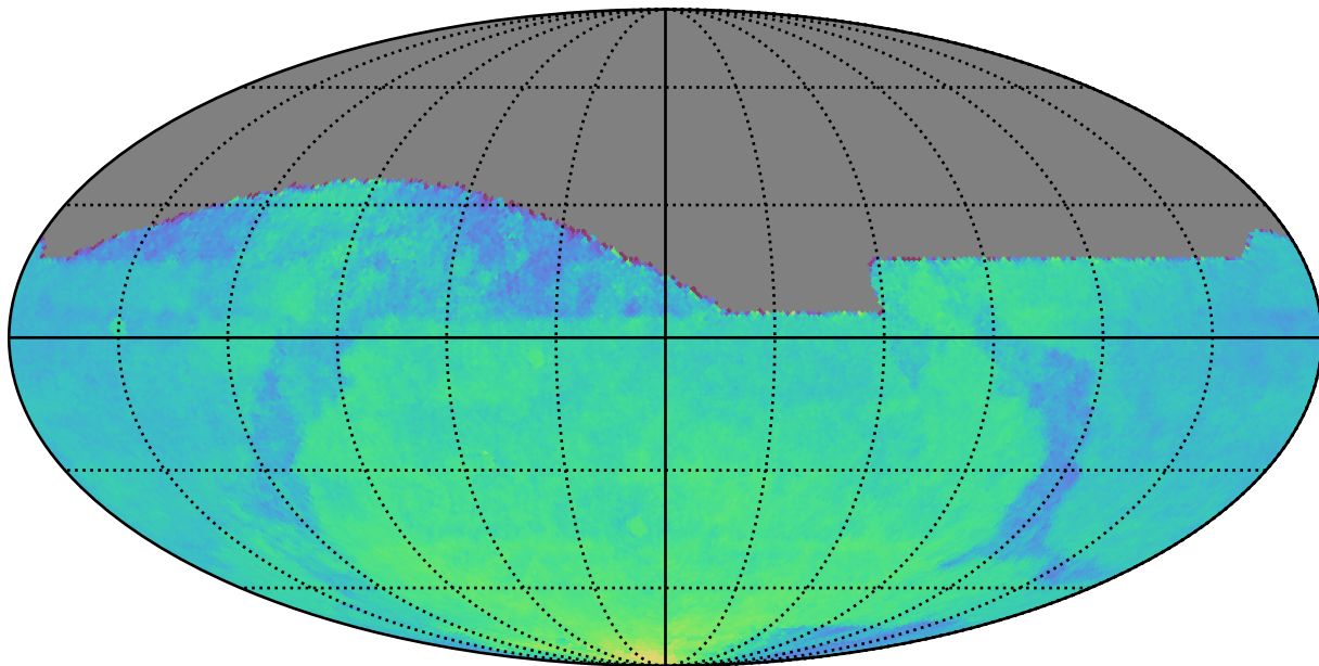
weather_cloudso30v3.4_10yrs All sky: Parallax Coverage @ 22.4
