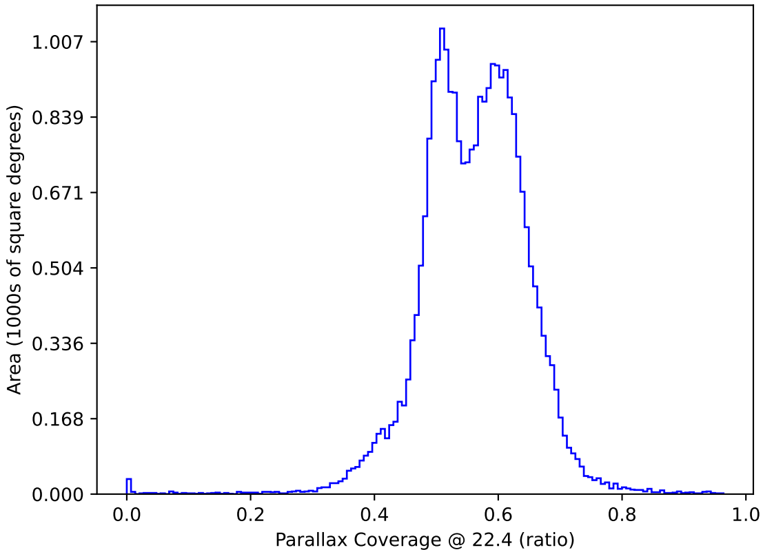
weather_cloudso30v3.4_10yrs All sky: Parallax Coverage @ 22.4
