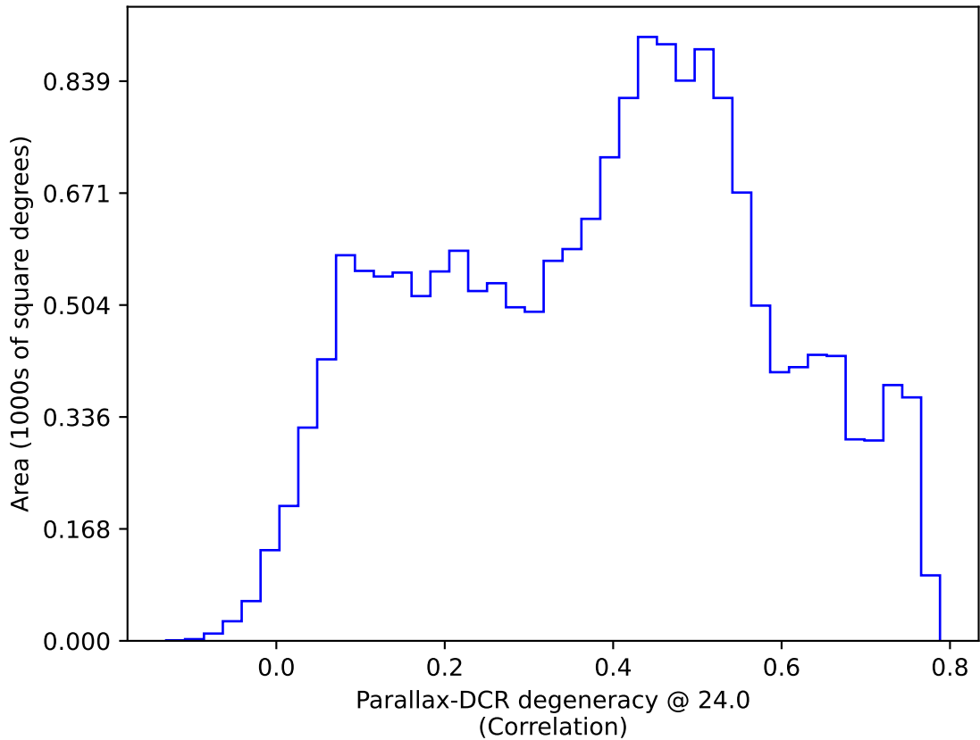
weather_cloudso30v3.4_10yrs WFD: Parallax-DCR degeneracy @ 24.0
