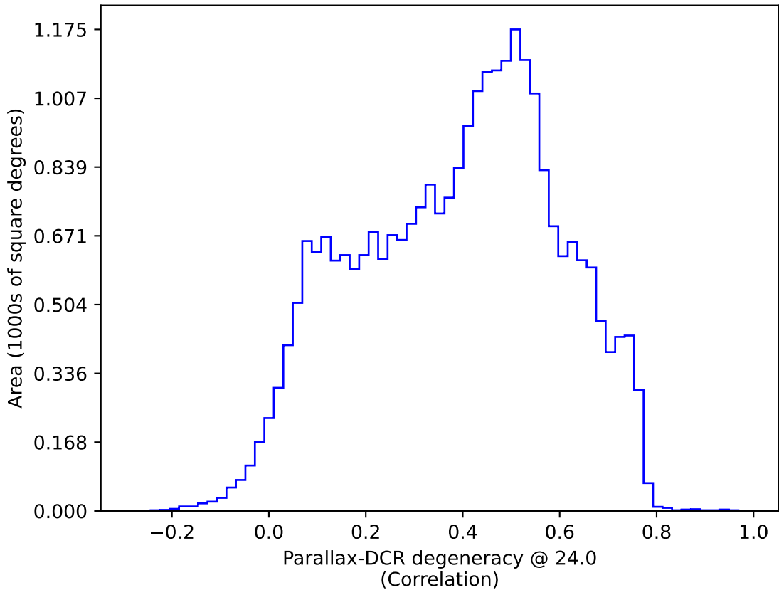
weather_cloudso30v3.4_10yrs All sky: Parallax-DCR degeneracy @ 24.0
