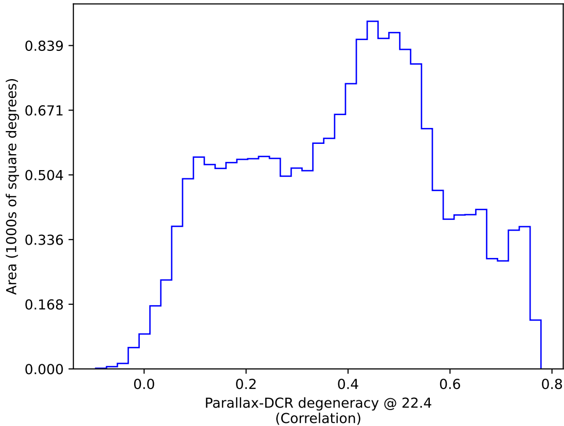
weather_cloudso30v3.4_10yrs WFD: Parallax-DCR degeneracy @ 22.4
