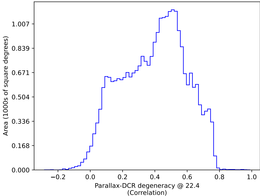
weather_cloudso30v3.4_10yrs All sky: Parallax-DCR degeneracy @ 22.4
