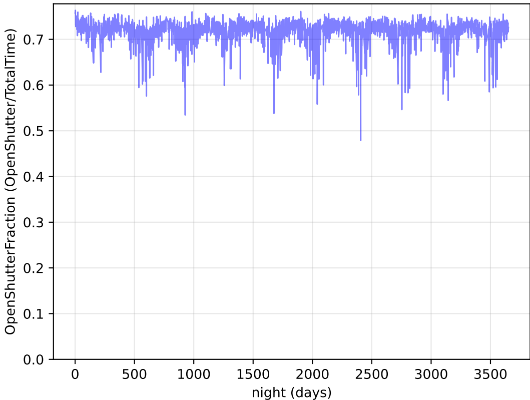
weather_cloudso30v3.4_10yrs Per night: OpenShutterFraction
