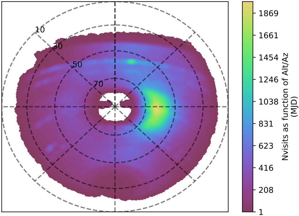
weather_cloudso30v3.4_10yrs y band: Nvisits as function of Alt/Az
