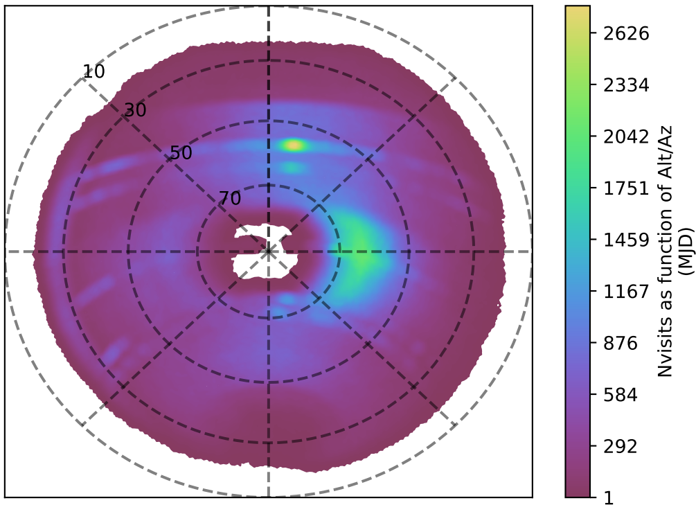
weather_cloudso30v3.4_10yrs r band: Nvisits as function of Alt/Az
